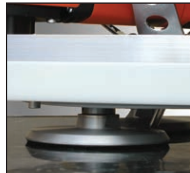
One of three 5" grinding platens (Velcro® surface)
