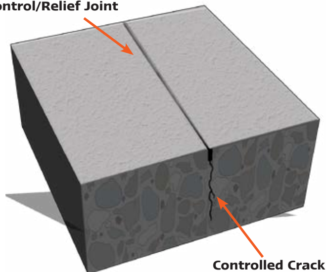
Control/Relief Joint
